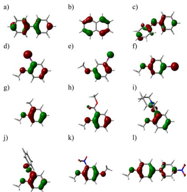
Figure 3. The lowest unoccupied molecular orbitals of radical cation of (a) 3, (b) 5, (c) 7, (d) 10, (e) 12, (f) 15, (g) 17, (h) 19, (i) 22, (j) 24, (k) 26, and (l) 29 obtained by DFT calculations (UB3LYP/6-31G*).
